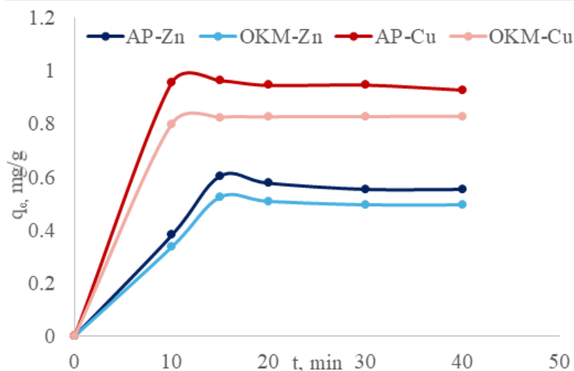
Fig.4 Dependence of adsorption capacity on adsorbent-adsorbate contact time ( c_0 = 10 \text{ mg/dm}^3 )
