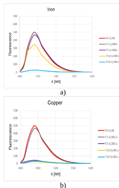
Fig.6 Relative fluorescence intensity of cotton fabrics treated with 0.08% FWA without and with the addition of a) iron (Fe) and b) copper (Cu) ions
