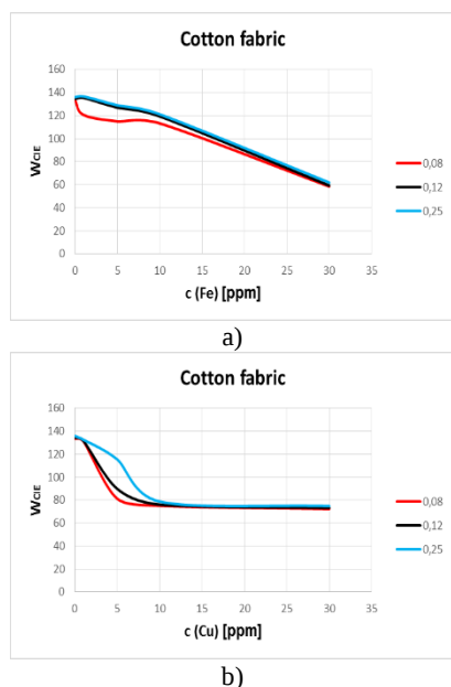
Fig.10 The whiteness degree of cotton fabric after treatment with different concentrations of FWA and the addition of different concentrations of a) iron and b) copper ions
