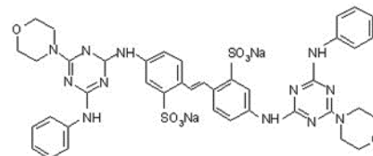
Fig.1 Stilbene derivative, 4,4'-bis-(triazinylamino)stilbene-2,2'-disulfonate [14]
