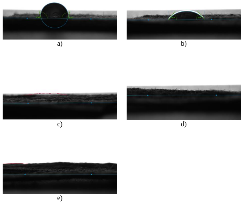
Fig.2 Screenshots from the DSA30S software when determining the contact angle on a white cotton fabric: a) unwashed, and after b) 1 st , c) 5 th , d) 10 th , and e) 15 th washing cycle
