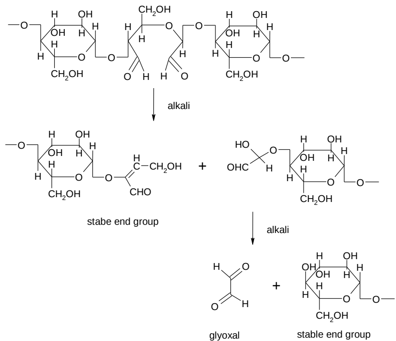
Fig.3 Alkaline hydrolysis of oxycellulose
