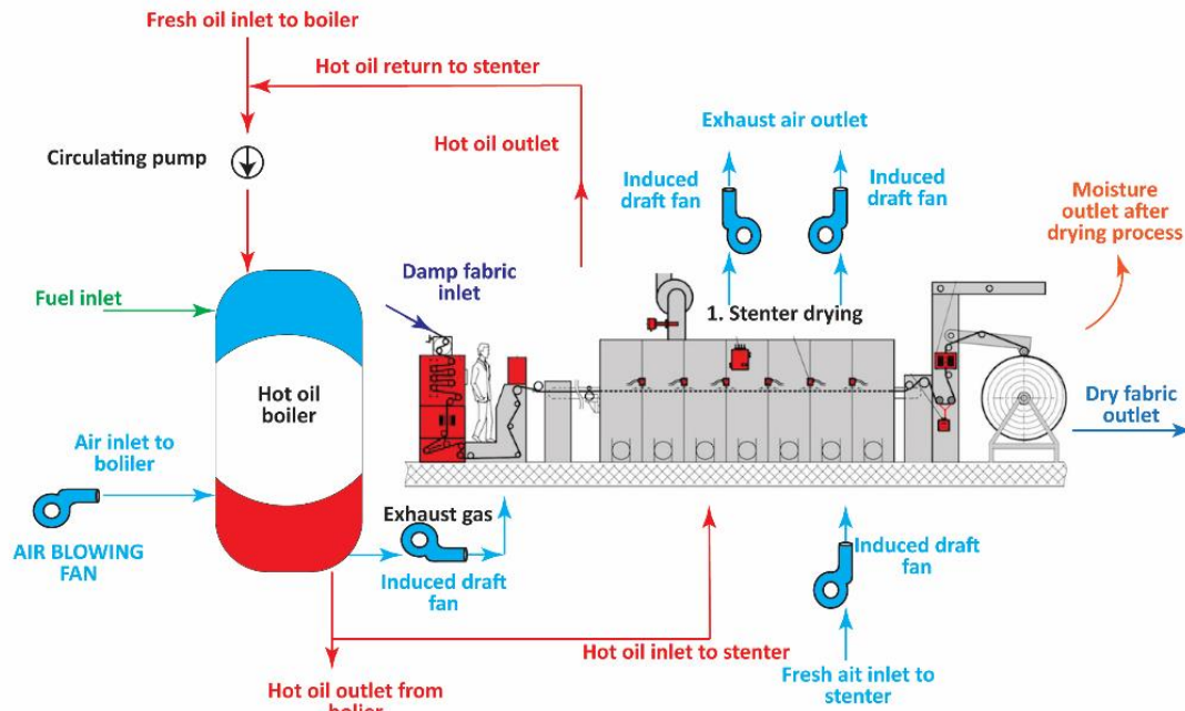
Fig.2 Stenter drying process with indirect heating
