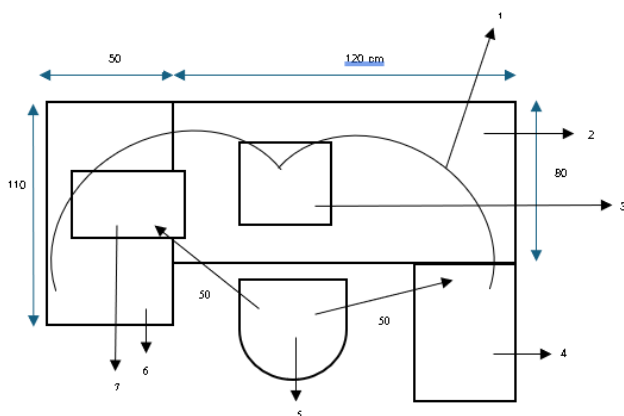
Fig.4 Workplace design for the technological operation of front 3 side overlook: 1-maximum reach zone; 2-sewing machine table; 3-head of the overlook machine; 4-table for putting down the pieces; 5-chair; 6-table on which bundles are placed; 7-front piece
